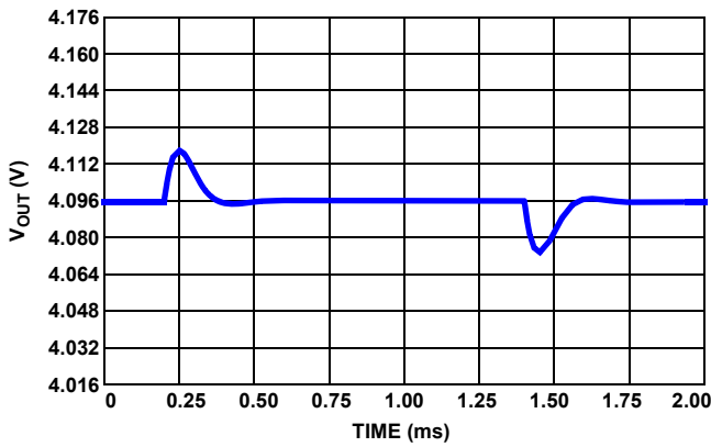
FIGURE 26. SIMULATED LOAD TRANSIENT ( \Delta I_L = 1\text{mA} )
